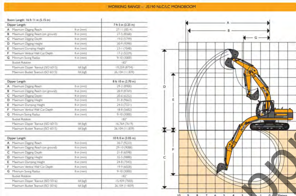
JCB JS 190 NC
